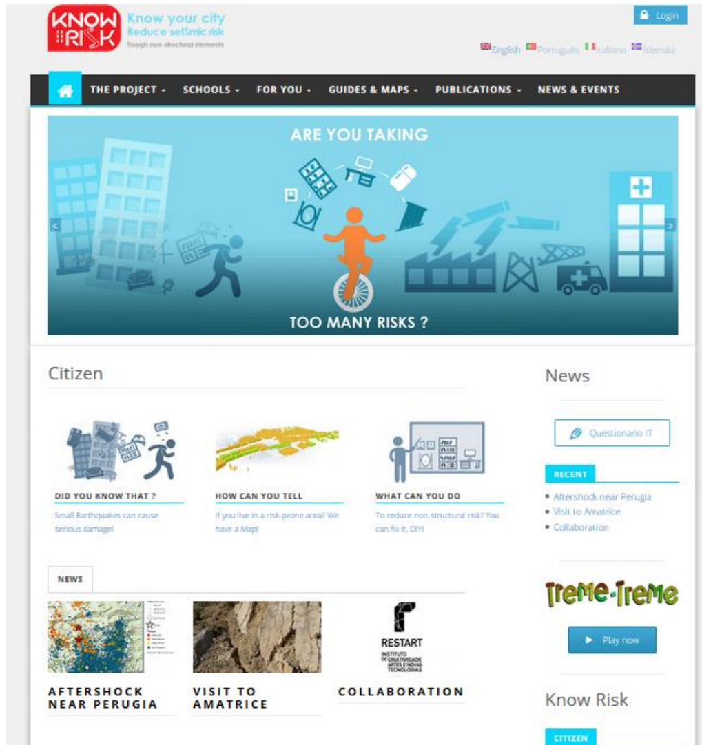
Figure 1. Homepage
