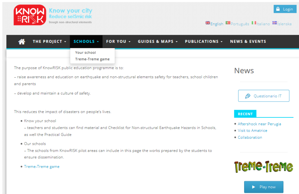
Figure 3. Schools page
