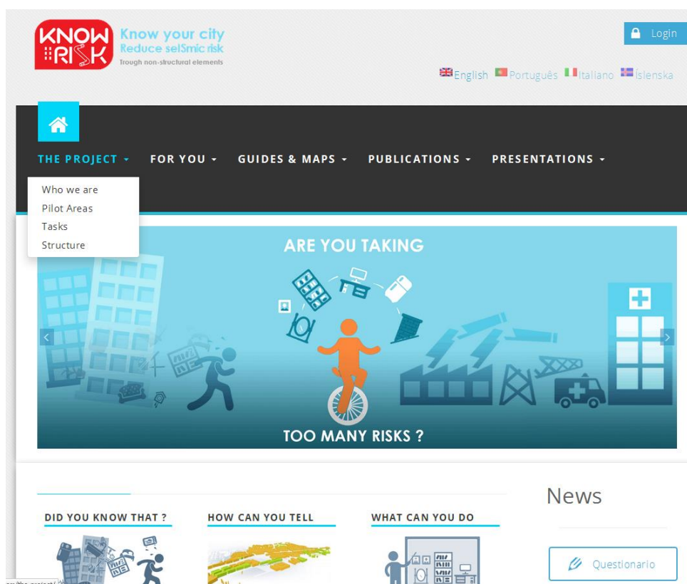
Figure 2. Project description
